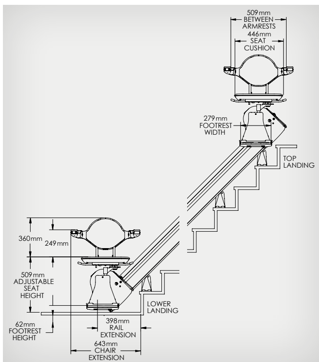
Front view lower and upper landing
