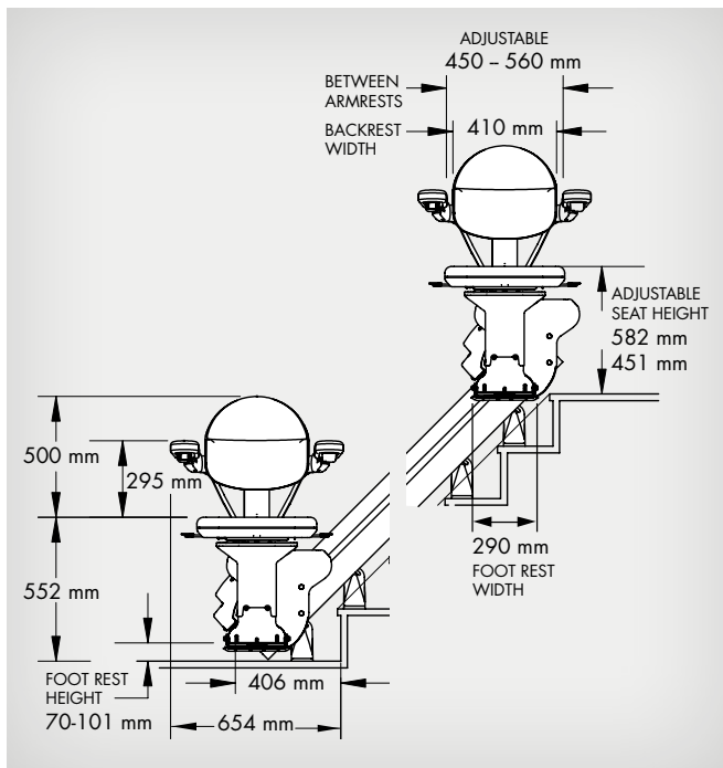
Front view lower and upper landing
