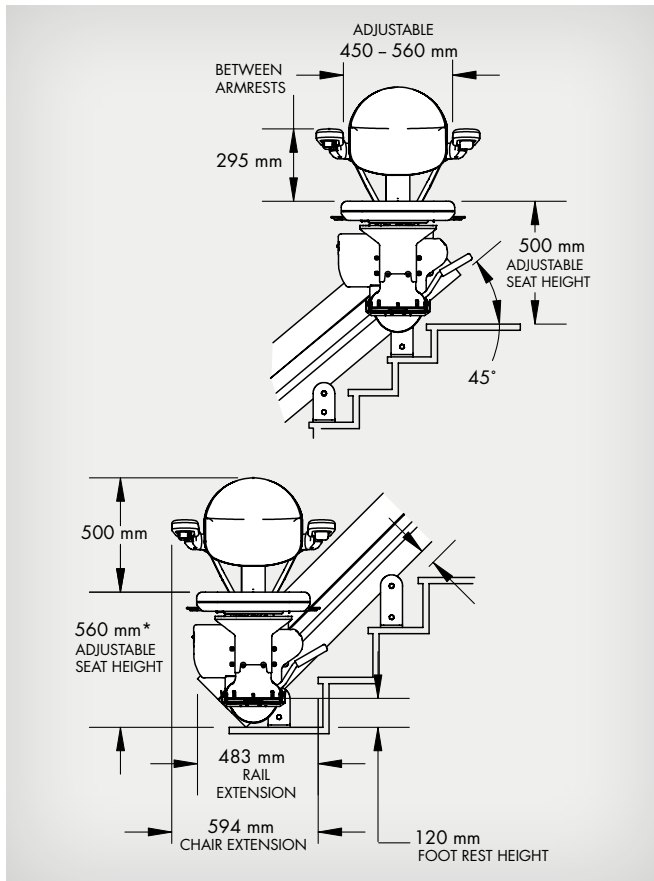
Front view lower and upper landing
