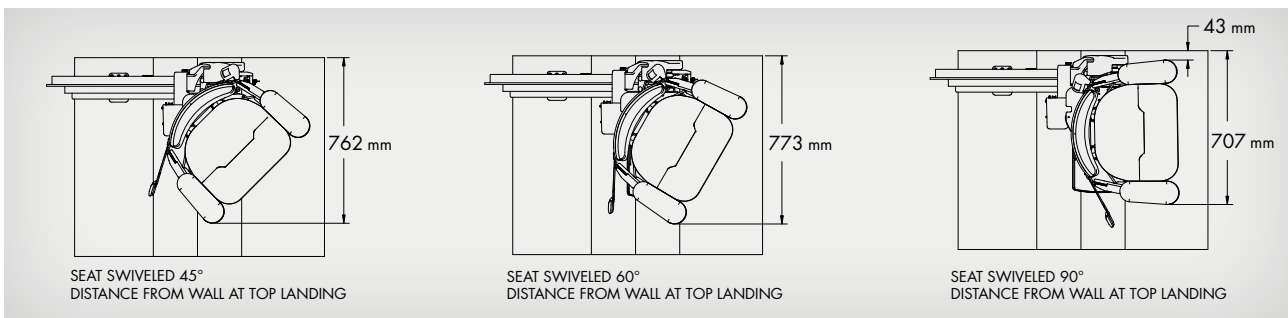
Top view
